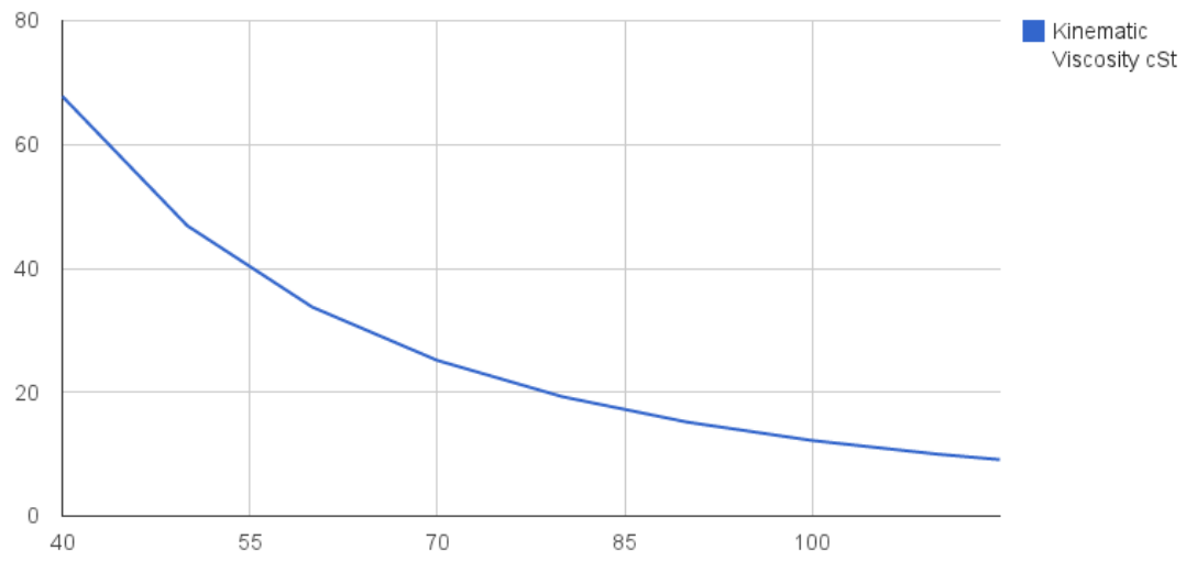
Mobil 1 0W30 ESP Kinematic Viscosity/ Temperature
